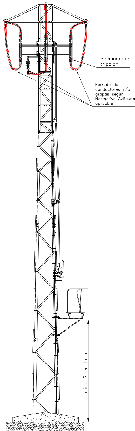
VISTA FRONTAL
