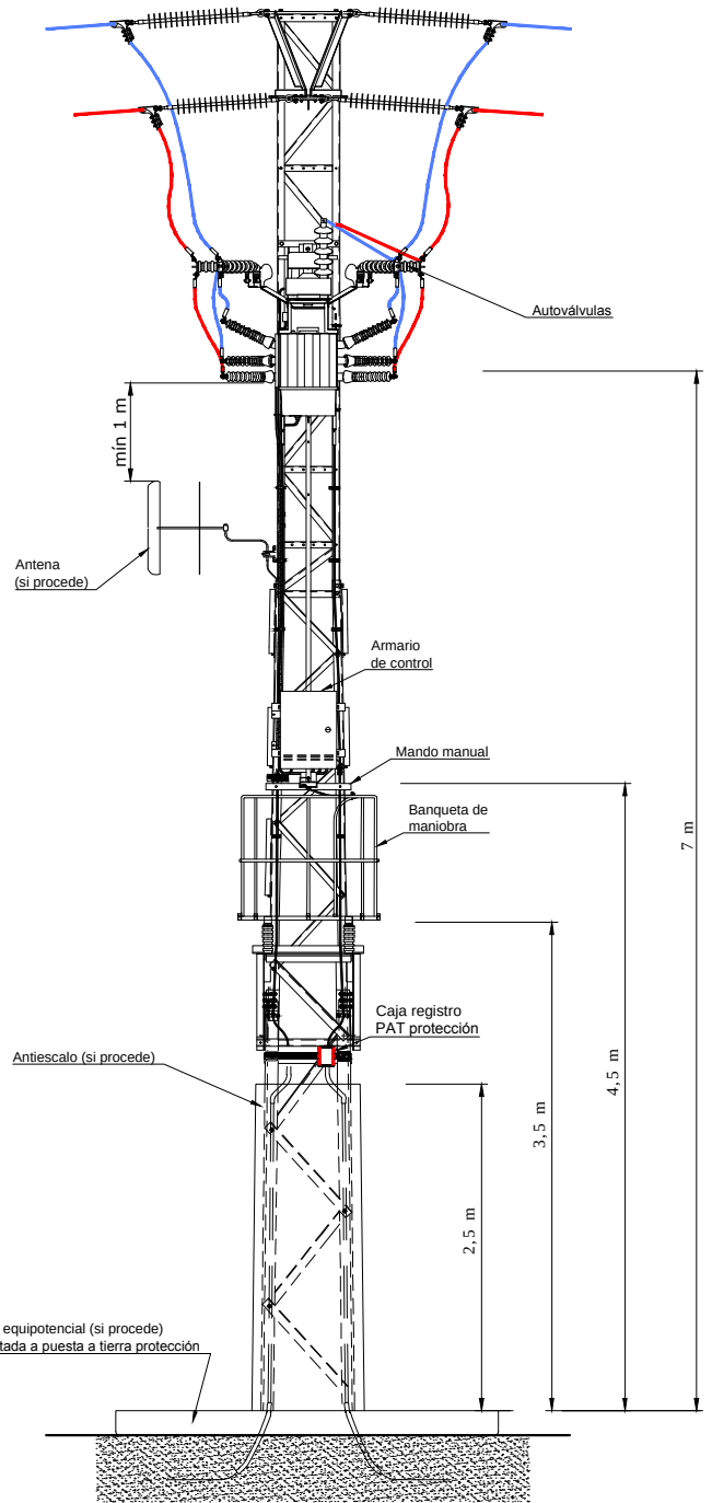
VISTA FRONTAL
