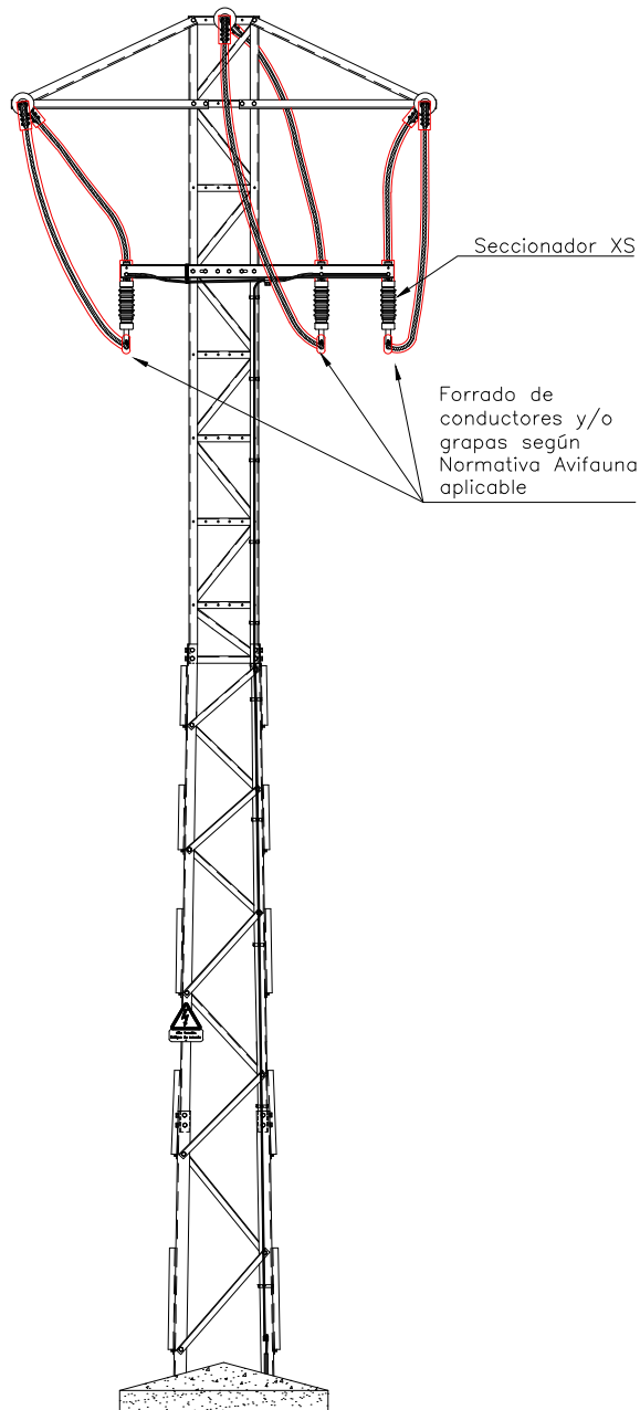
VISTA FRONTAL
