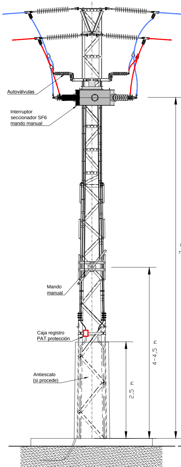
VISTA FRONTAL
