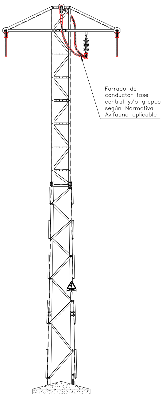
VISTA FRONTAL
